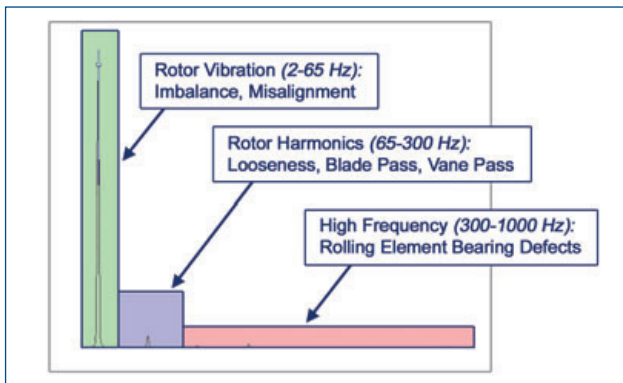
By dividing the spectrum into energy bands, we can isolate frequencies associated with different categories of faults.
