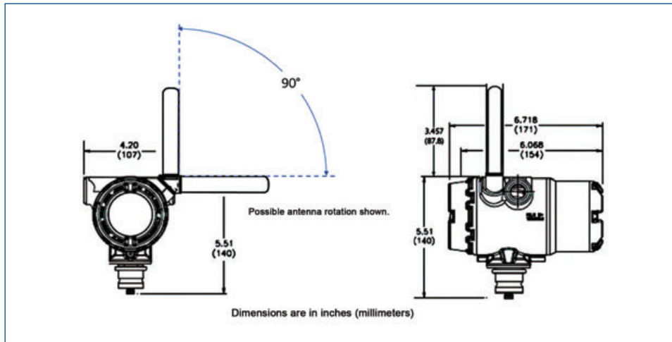
CSI 9420 dimensional drawing
