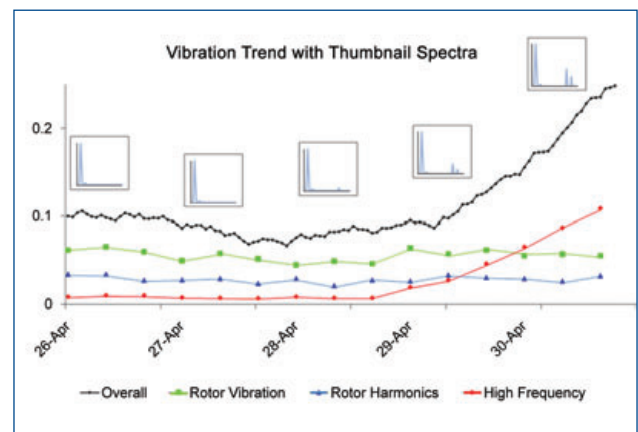
The trend of overall vibration suggests that machine health is deteriorating but without any indication as to the root cause. The trend of the high frequency energy band provides further insight, which can be confirmed by examining the thumbnail spectra.
